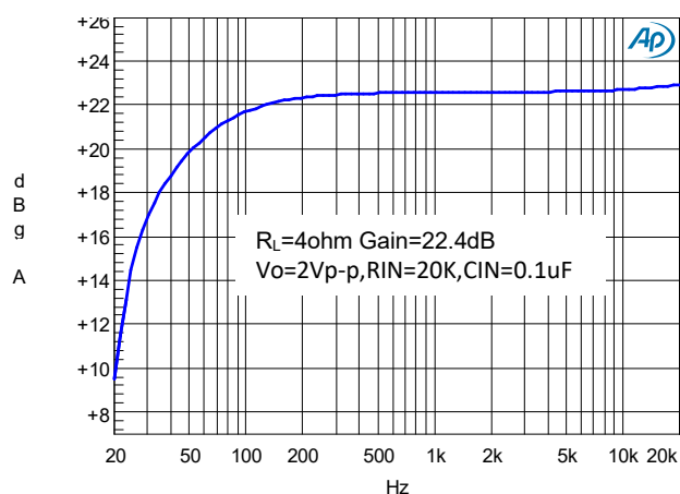
Frequency Response
